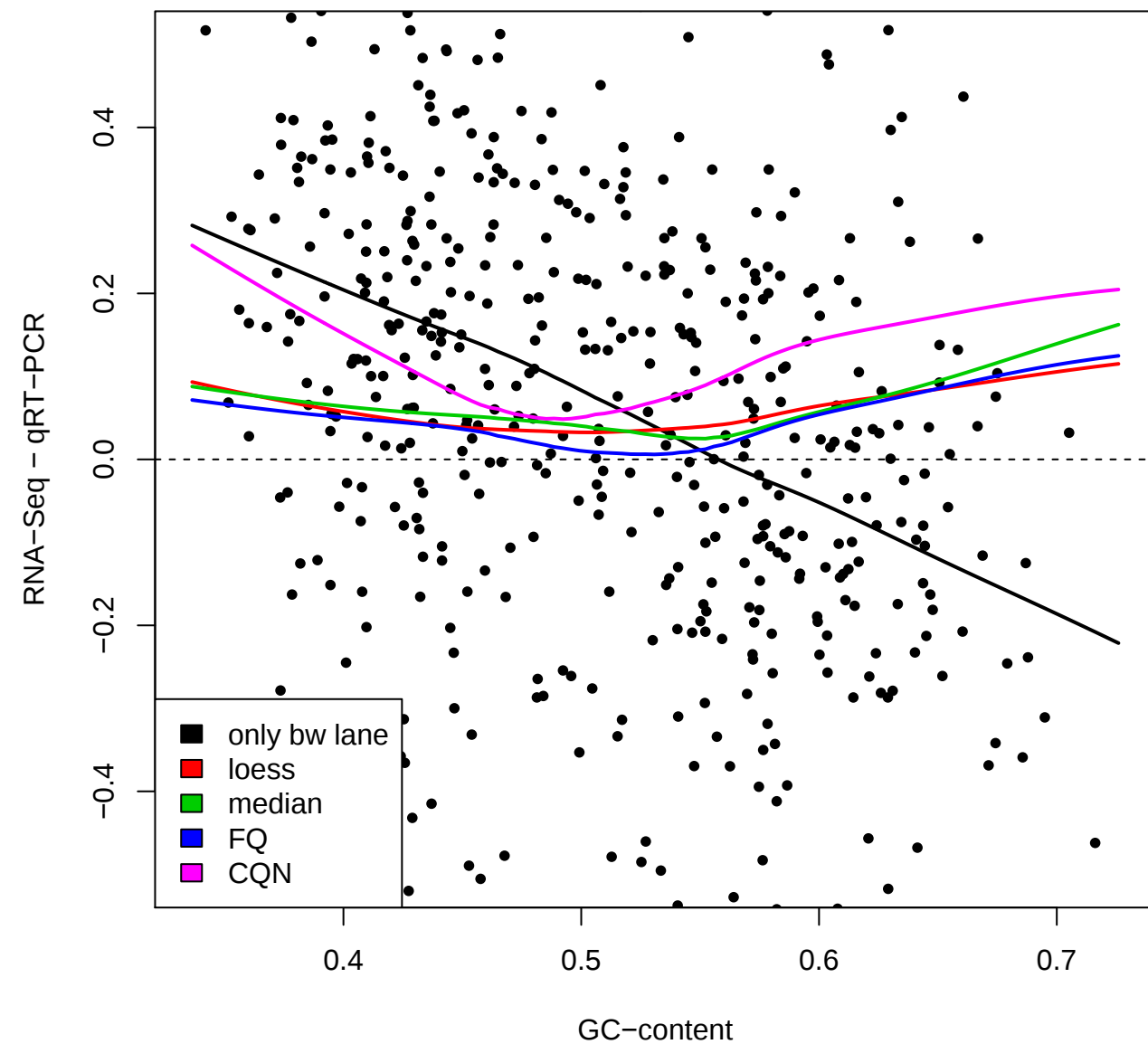
(b) Bias vs. GC-content
