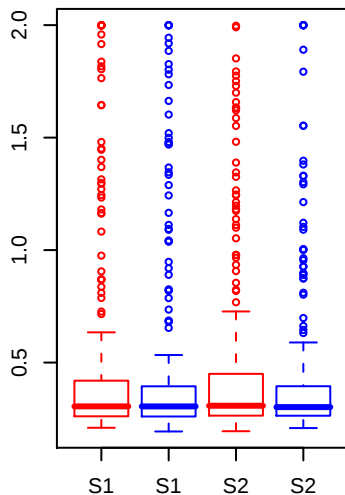
Time at epidemics peak
