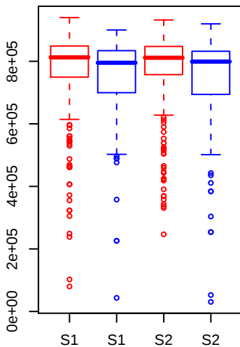
Sampled epidemics size
