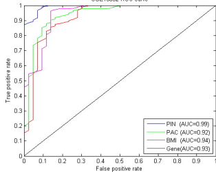
GSE15852 ROC curve
