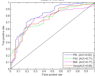
GSE6919 ROC curve
