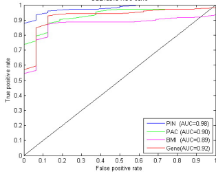
GSE16515 ROC curve
