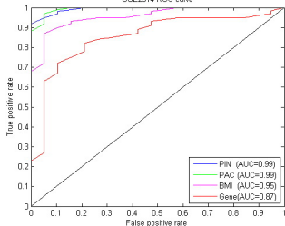
GSE2514 ROC curve
