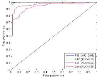
GSE10072 ROC curve
