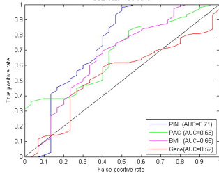
GSE19027 ROC curve
