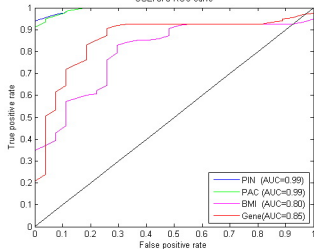
GSE7670 ROC curve
