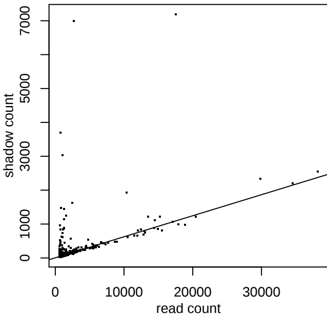
re-sequencing
