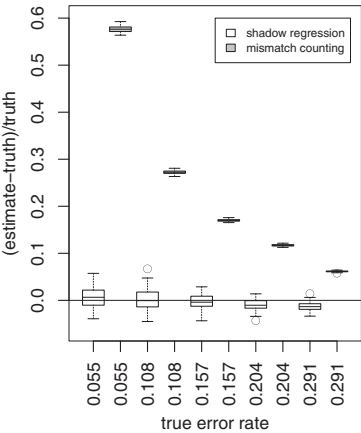
Simulation under independence
