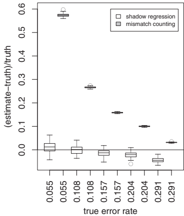
Simulation under dependence
