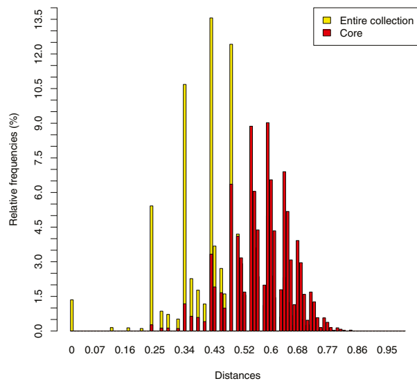
Distance distribution of large pea dataset mixedMR core (int=0.2)
