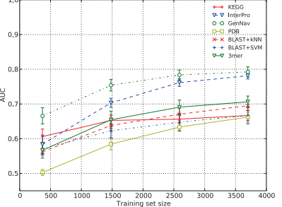
AUC by training size for Toxin
