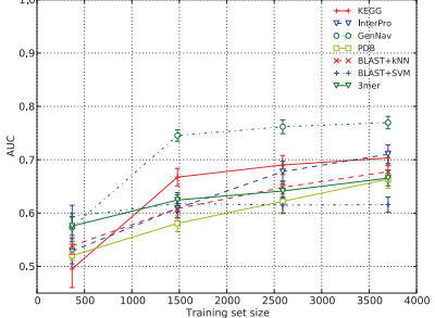
AUC by training size for Catalysis
