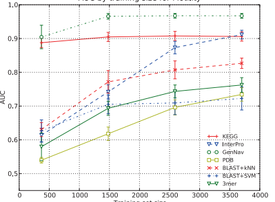
AUC by training size for Motility
