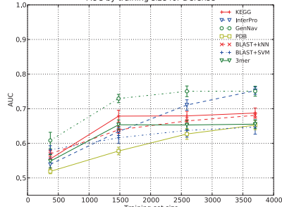
AUC by training size for Defense
