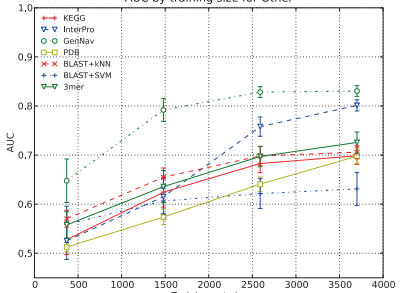
AUC by training size for Other
