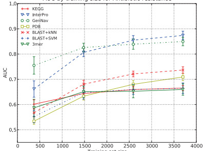
AUC by training size for Antibiotic resistance
