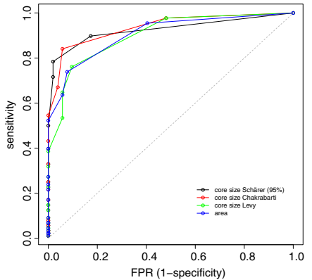
ROC curves for geometry predictors with Ponstingl datasets
