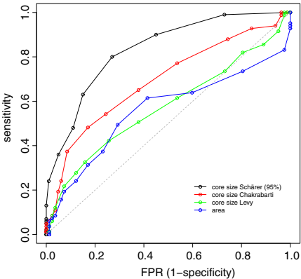
ROC curves for geometry predictors with DC datasets
