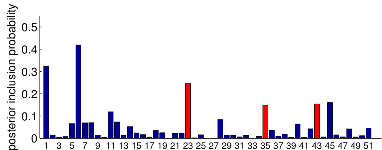
(c) Biologically informative prior – "incorrect"
