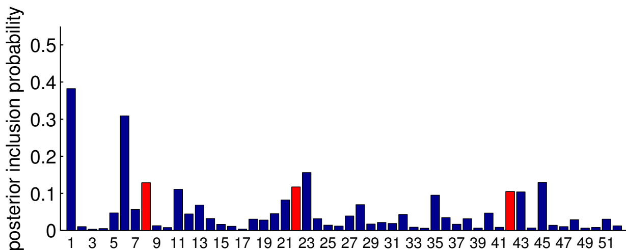
(b) Flat prior
