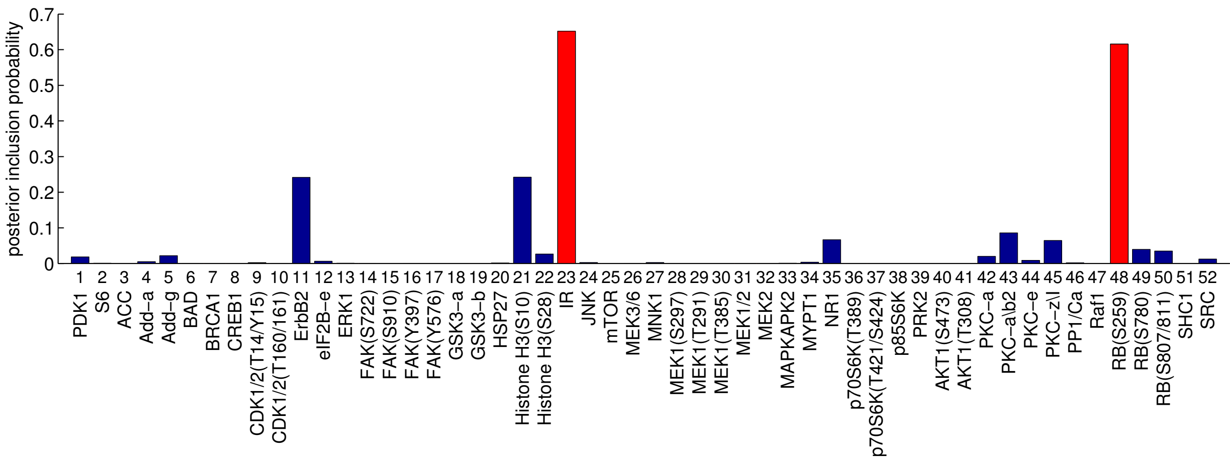
(a) Biologically informative prior – empirical Bayes
