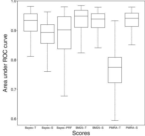
PHOSPHORYLATION
