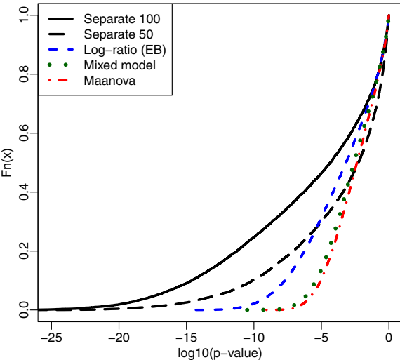
Cumulative Distribution of P-Values
