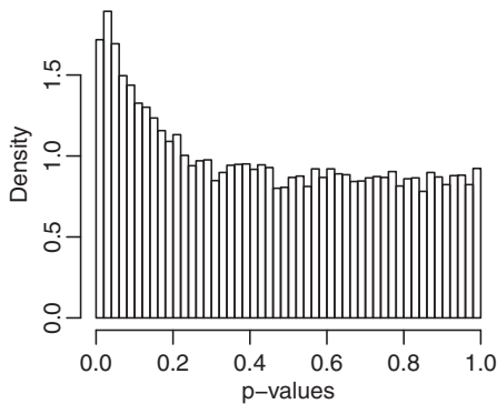
Mixed Model
