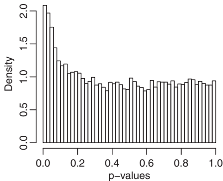
Log-Ratio
