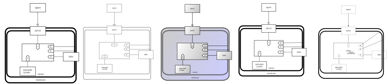
two_edges_between_two_activities.sbgm
