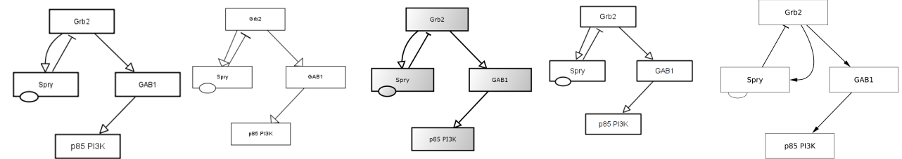
compartment.sbgm
