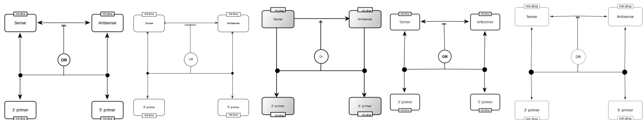
outcome-simplified.sbgm
