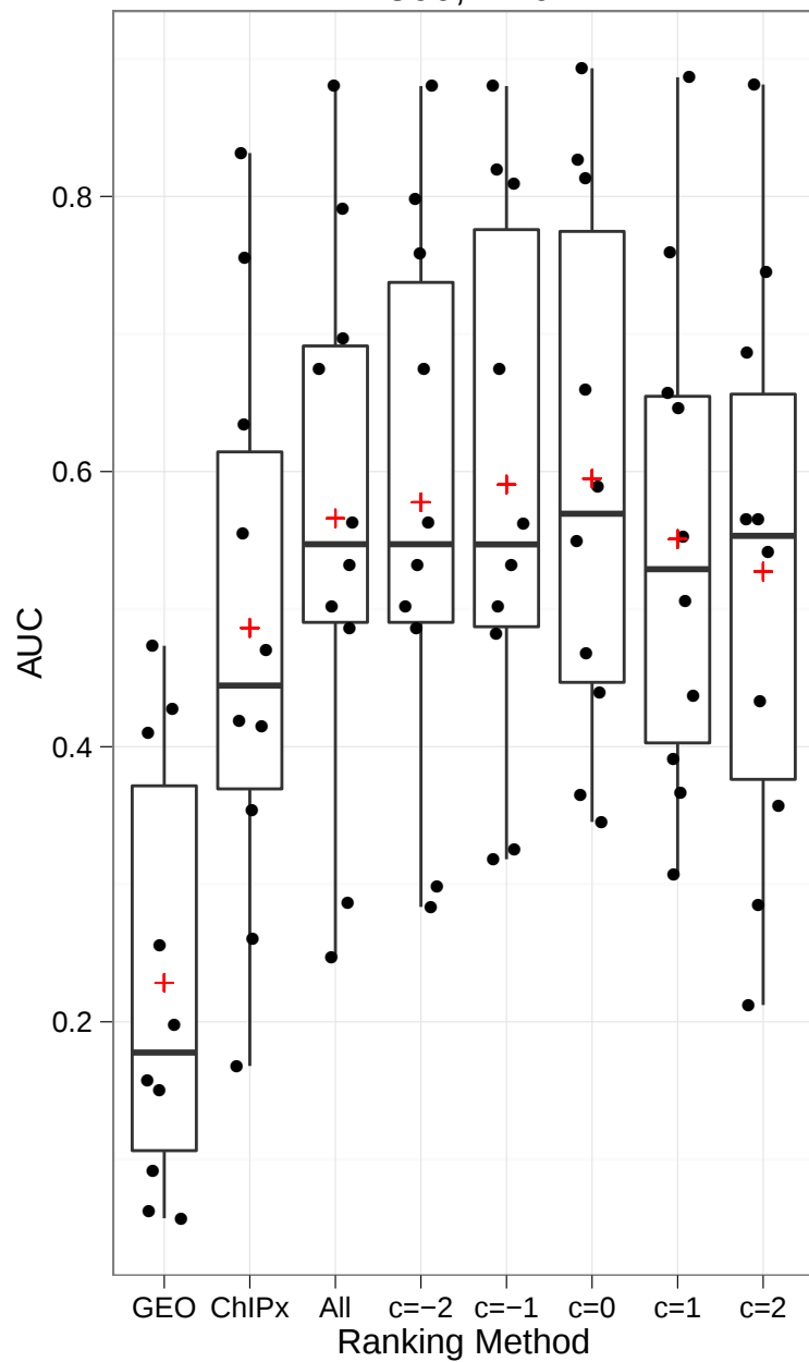
n=500, w=0.1
