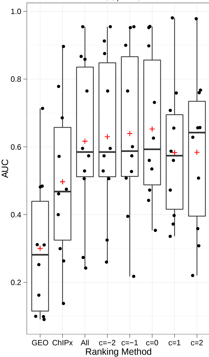
n=100, w=0.1
