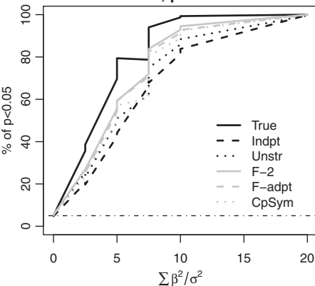
Cov=0.1; permutation
