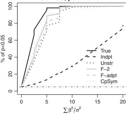
Cov=0.5; permutation
