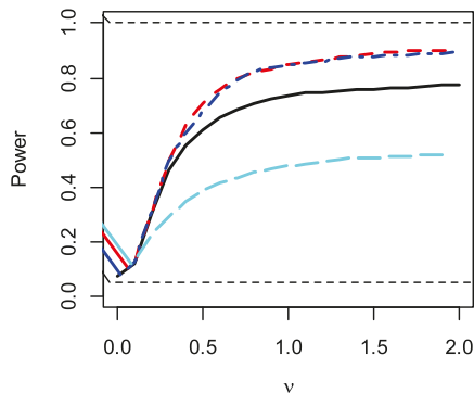
Power at \alpha=0.05 , \rho=0.9
