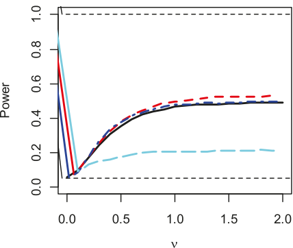
Power at \alpha=0.05 , \rho=0.6
