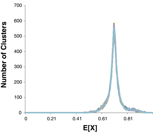
10^5 Randomizations
