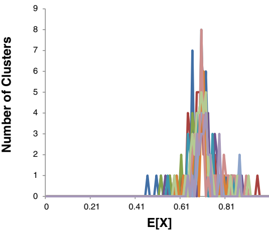
10^3 Randomizations
