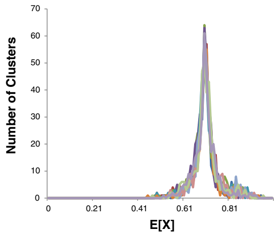
10^4 Randomizations
