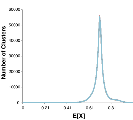
10^5 Randomizations
