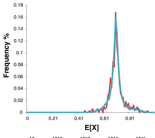
Threshold Estimation
