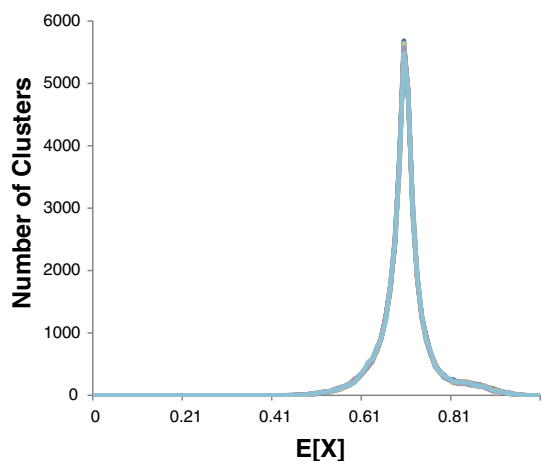
Threshold Estimation
