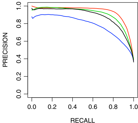
Precision Recall
