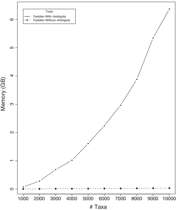
Memory comparison of Fastdist
