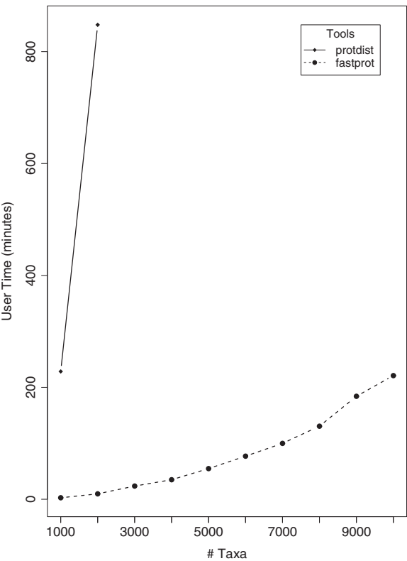
Time comparison of Protdist vs Fastprot
