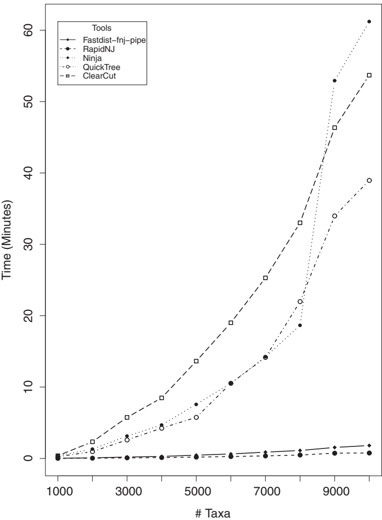
Dataset-1: Time Comparison
