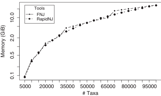
Dataset-2: Memory Comparison of FNJ vs RapidNJ
