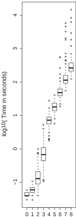
30-node net
