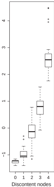
40-node net
