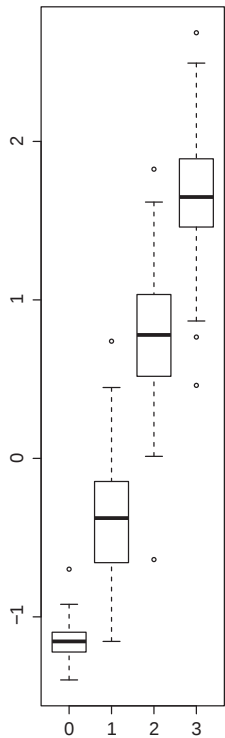
50-node net
