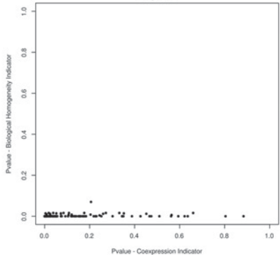
Integration
