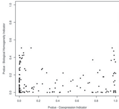
WGCNA
