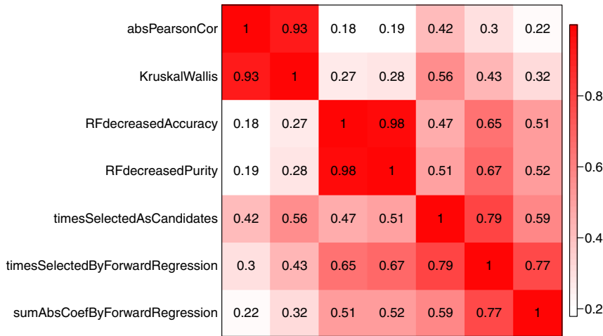
Relationship of feature ranking methods
