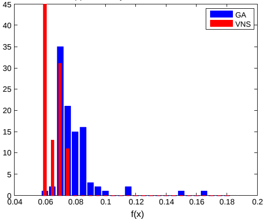
Best f(x) obtained by VNS and GA over 100 runs
