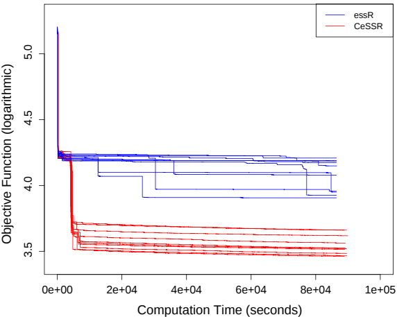
LSGO benchmark, F10: cooperative (every 1h) vs. non cooperative threads
