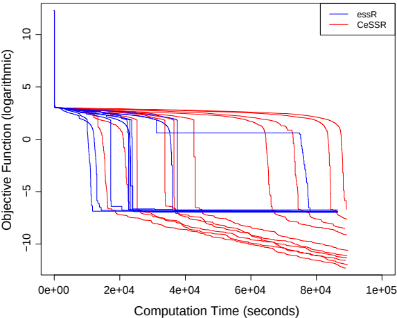
LSGO benchmark, F20: cooperative (every 1h) vs. non cooperative threads
