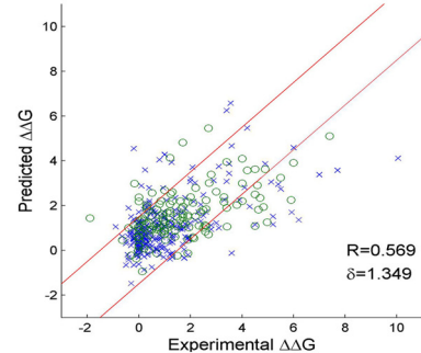
(a) \Delta\Delta G prediction by \beta ACV_{ASA}
