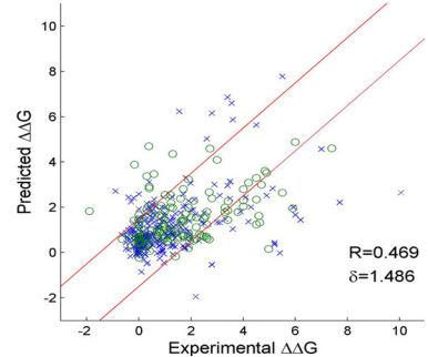
(c) \Delta\Delta G prediction by non\beta ACV_{ASA} based on non- \beta contacts
