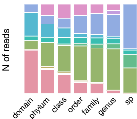
Real - Sample B
