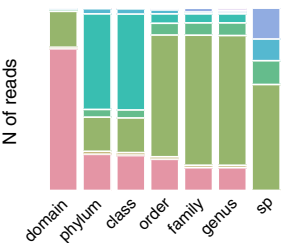
Sim - Bacterial genomes
