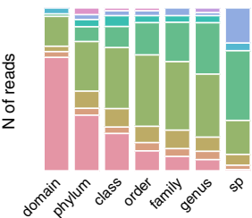
Real - Sample A
