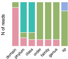
Sim - Bacterial genomes (dominant)
