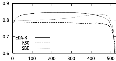
528 features
