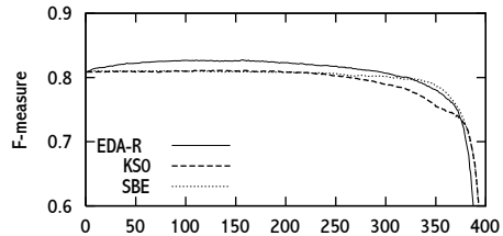
400 features
