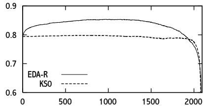
2096 features
