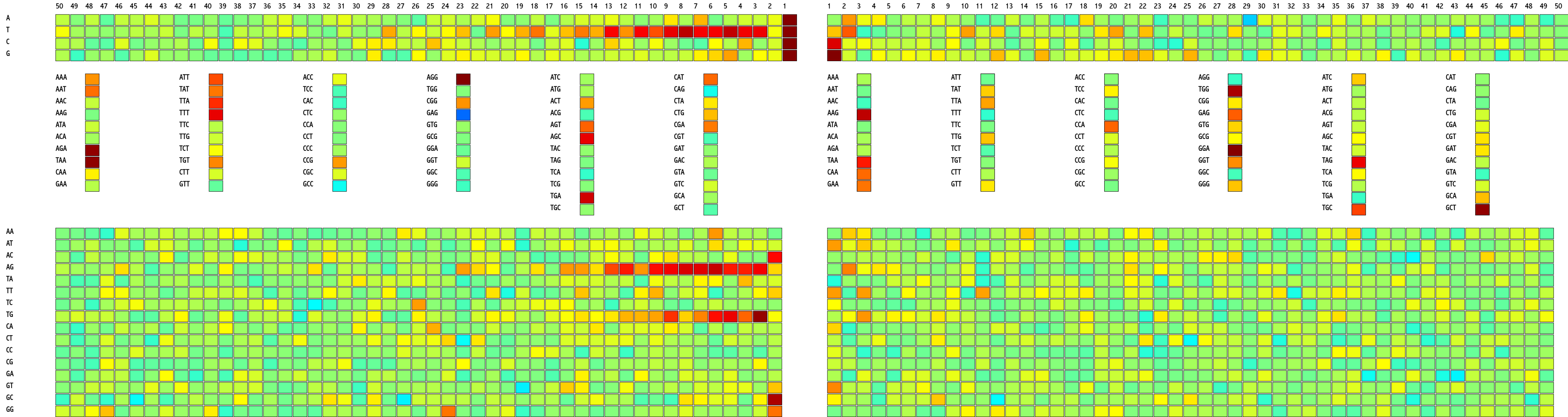
Acceptors : 2096 features
