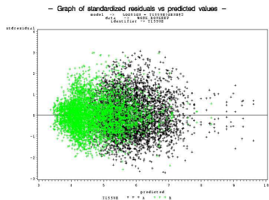
(a) Residuals versus predicted
