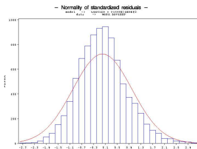
(b) Gaussian distribution of residuals
