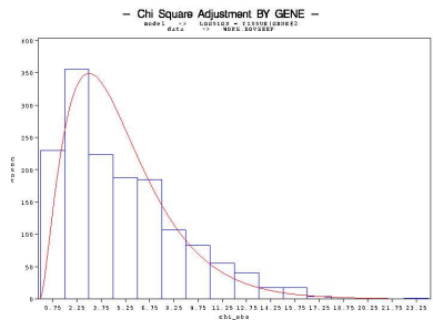
(c) Distribution chi2 of variances
