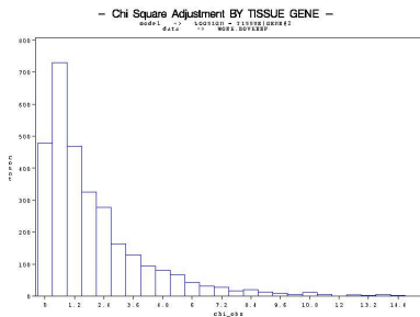
(c) Distribution chi2 of variances
