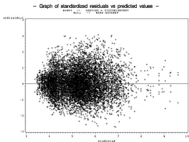
(a) Residuals versus predicted
