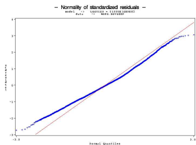
(b) Gaussian distribution of residuals
