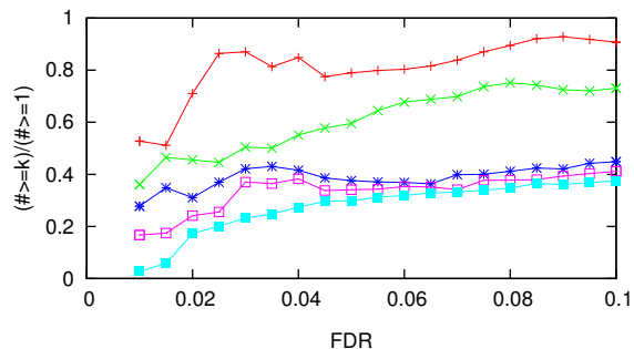
Colon rank-sum statistic
