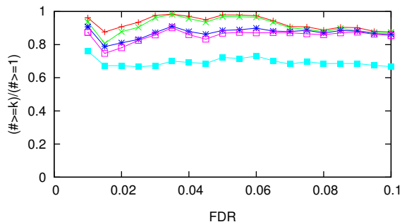
Ovary rank-sum statistic
