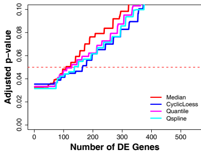
Wilcoxon test
