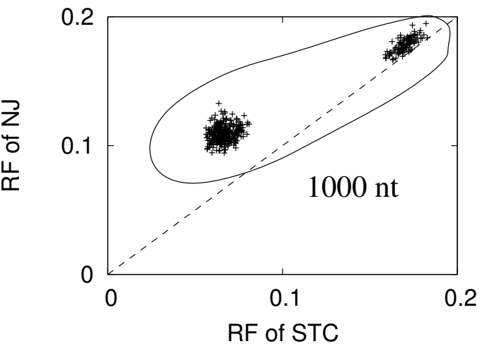
(c) STC versus NJ (5000 taxa)
