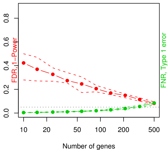
Sample size= 40
