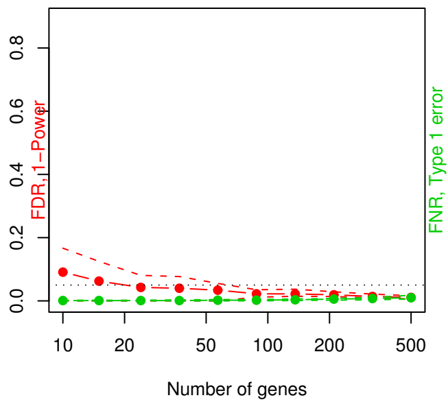
Sample size= 100
