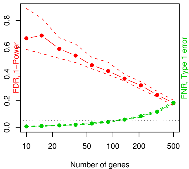
Sample size= 20
