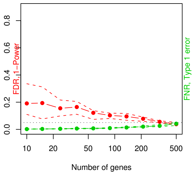
Sample size= 60
