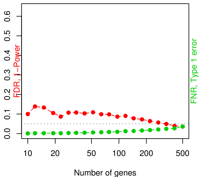
Sample size= 60
