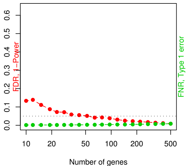
Sample size= 100
