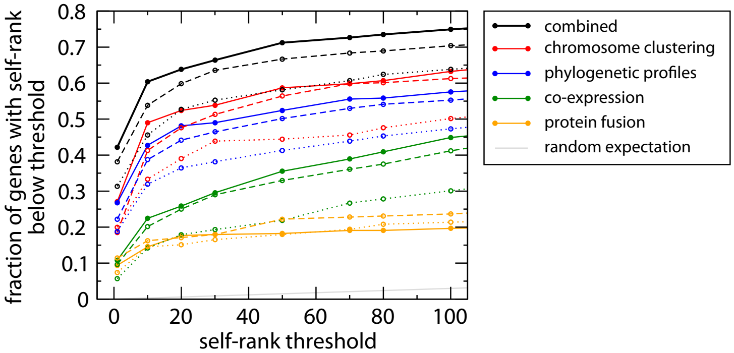
Effects of metabolite weighting and association-rank rescaling corrections. E. coli self-rank performance is shown for individual types of association evidence and for their combination. Performance based on metabolite weighting and association-rank rescaling corrections is shown in solid lines, with association-rank correction only in dashed lines, and without either correction in dotted lines. Prediction were generated using using ADT classifier (with 10 fold validation) based on association scores to 3 layers of the metabolic network neighborhood.
