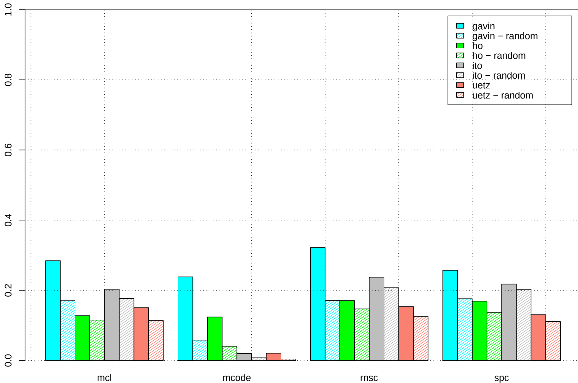
Weighted geometrical accuracy of tested algorithms applied to large scale interaction data sets
