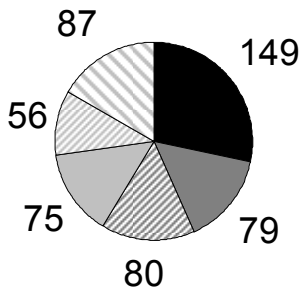
Kinase
