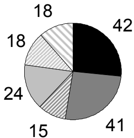
Phosphatase
