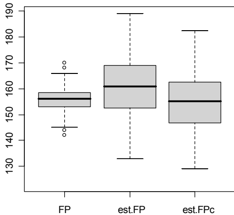
symmetric cutoff method
