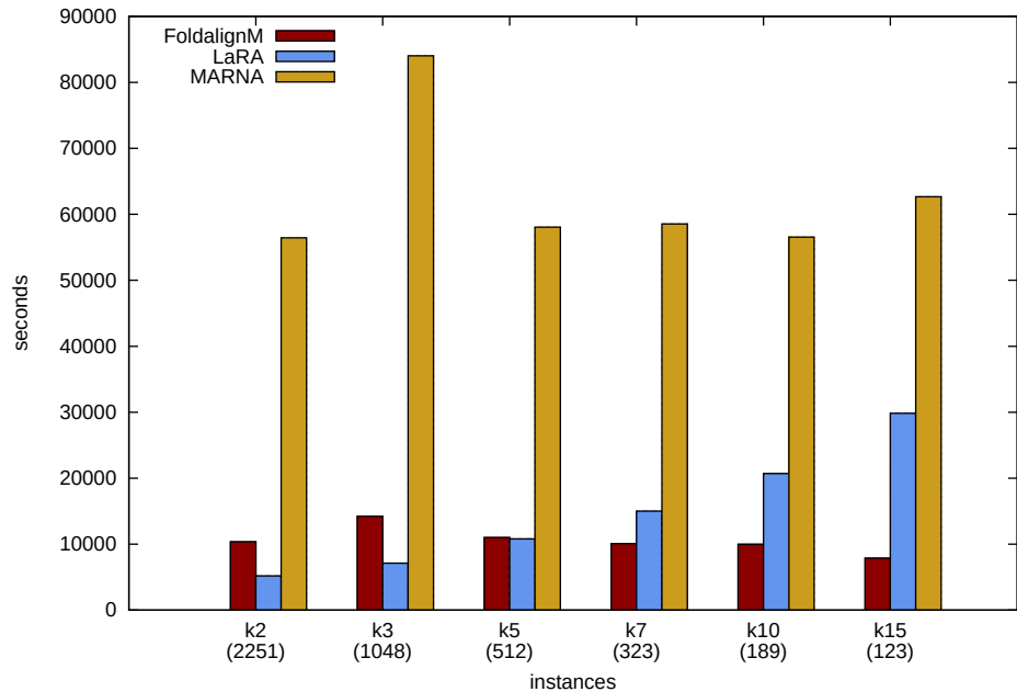
Comparison of running times
