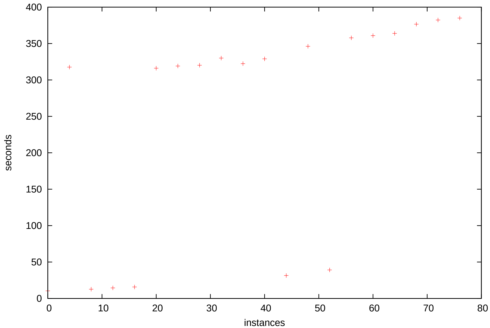
dlvhex performance
