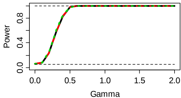
Power at \alpha=0.05, r=0
