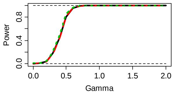
Power at \alpha=0.0025, r=0
