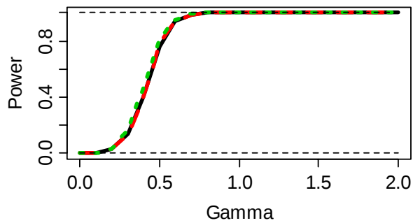
Power at \alpha=0.001, r=0
