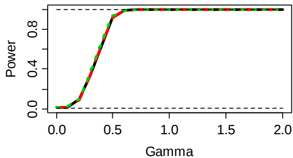
Power at \alpha=0.01, r=0
