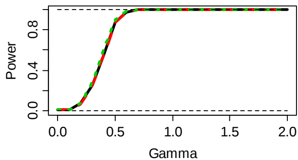
Power at \alpha=0.005, r=0
