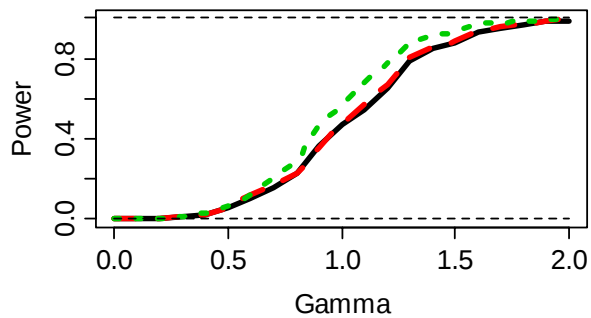
Power at \alpha=0.001, r=0.9
