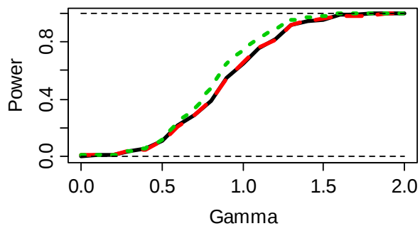
Power at \alpha=0.005, r=0.9
