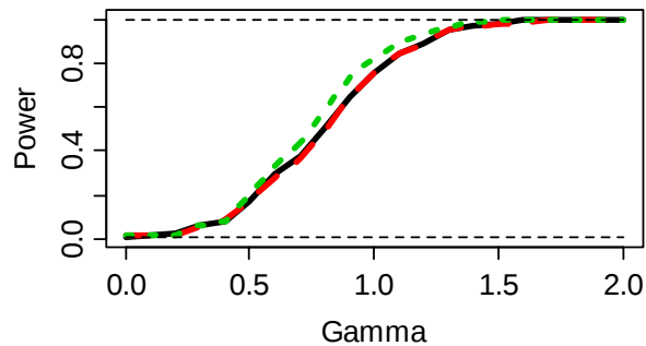
Power at \alpha=0.0025, r=0.9
