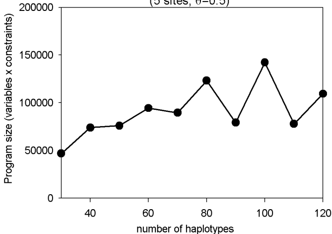
(c) Peak Program Size vs. Number of Sequences (5 sites, \theta=0.5 )
