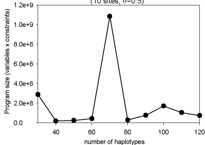
(d) Peak Program Size vs. Number of Sequences (10 sites, \theta=0.5 )
