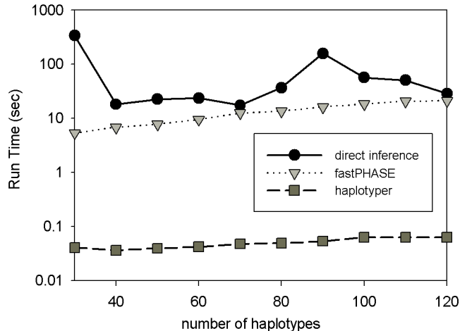
(b) Run Time vs. Number of Sequences (10 sites, \theta=0.5 )
