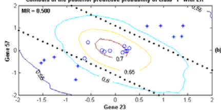
Contours of the posterior predictive probability of class "1" with GK(0.01)
