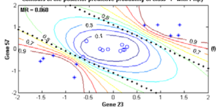
Contours of the posterior predictive probability of class "1" with PK(2)
