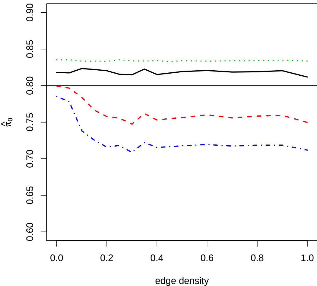
\pi_0 estimation under dependence
